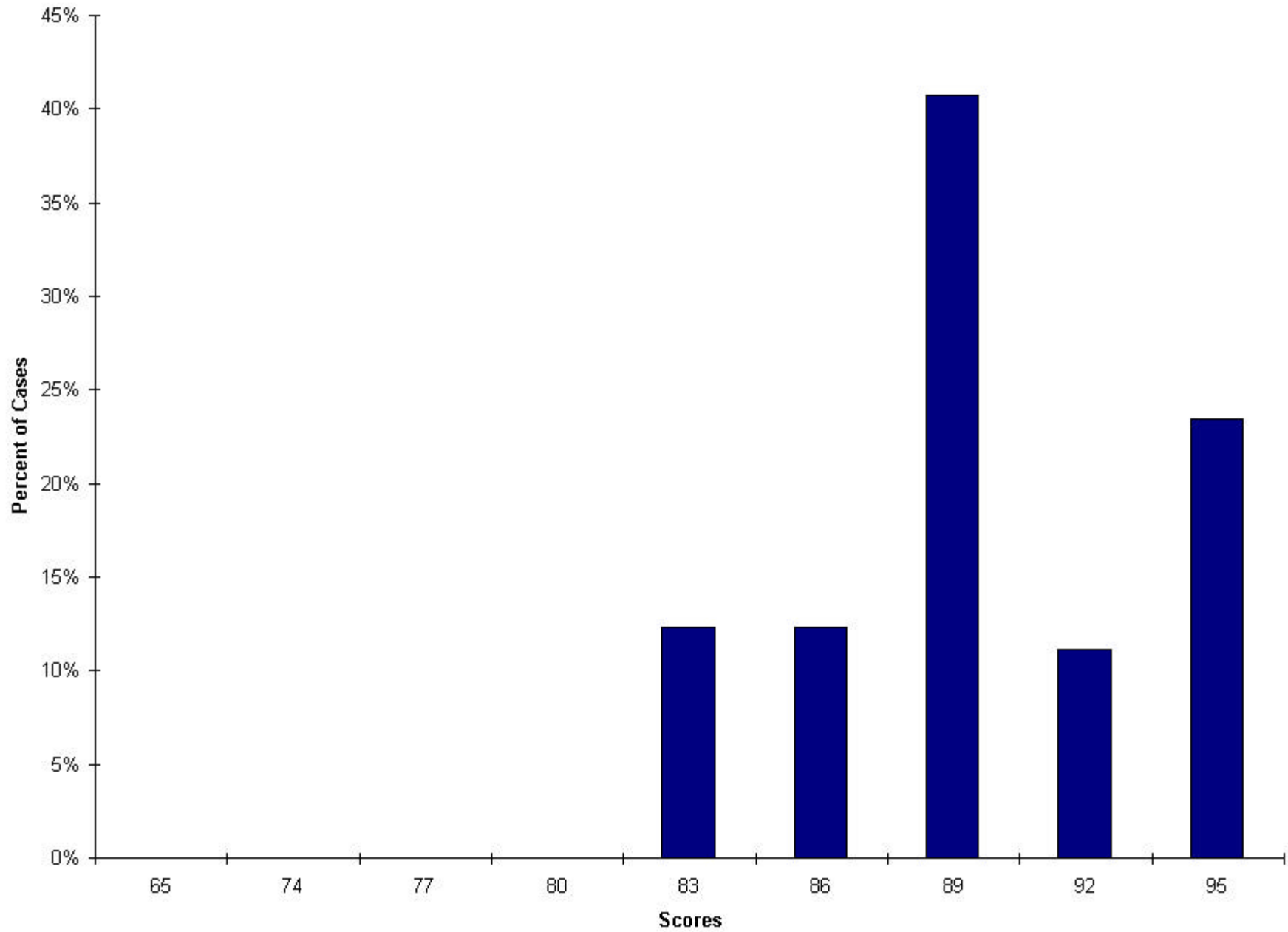
FIN 423 Case 2, Spring 1996 Mean = 88.8, Std = 3.8, Median = 88, N = 81
